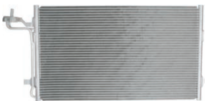
260489 Condenser Replacing: 9124389, 8623401, 4N5H19710BF, 31356000, 31292022 Servicing: Volvo Dryer w/o NB! Inlet/outlet has a different diameter. A: 376.00 B: 660.00 C: 20.00 mm
