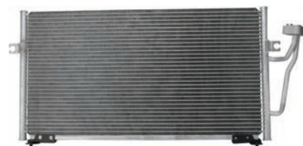
260076 Condenser Replacing: MR460269, MB958166 Servicing: Mitsubishi Dryer w/o A: 365.00 B: 740.00 C: 100.00 mm
