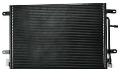
260068 Condenser Replacing: 8E0260403Q, 8E0260403N, 8E0260403L, 8E0260403K, 8E0260403J, 8E0260403H Servicing: Audi Dryer w/o A: 408.00 B: 615.00 C: 20.00 mm
