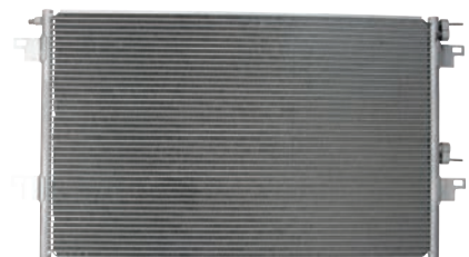
260460 Condenser Replacing: 8200033733 Servicing: Renault Dryer w/o A: 430.00 B: 695.00 C: 20.00 mm
