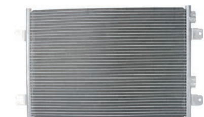
260461 Condenser Replacing: 8200557066, 8200191738, 8200182361 Servicing: Dacia, Renault Dryer w/o A: 392.00 B: 570.00 C: 20.00 mm
