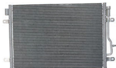
260066 Condenser Replacing: 8E0260403B, 8E0260403A Servicing: Audi Dryer w/o A: 410.00 B: 615.00 C: 20.00 mm
