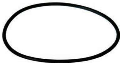
251260 O-ring ID 82.22, Thickness 2.62, Material Nioprene
