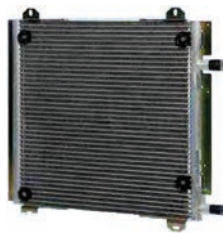
260458 Condenser Replacing: 7700433077, 7700428315 Servicing: Renault Dryer w/o A: 390.00 B: 422.00 C: 20.00 mm
