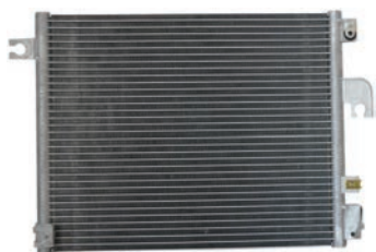
260398 Condenser Replacing: 9760605500, 97606-05500 Servicing: Hyundai Dryer w/o A: 350.00 B: 445.00 C: 18.00 mm
