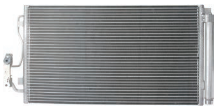
260725 Condenser Replacing: 9288940, 9218121, 64509335362, 64509288940, 64509218121, 64504270545 Servicing: BMW, MG Dryer w/ A: 355.00 B: 640.00 C: 20.00 mm
