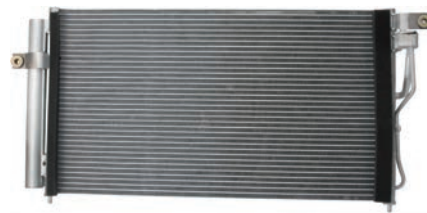
260941 Condenser Replacing: 97606-1E000 Servicing: Hyundai Dryer w/ A: 361.00 B: 635.00 C: 20.00 mm
