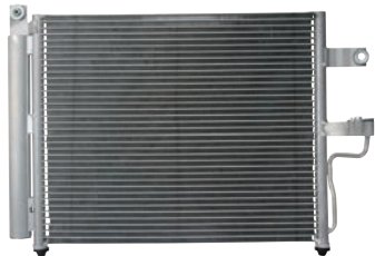
260722 Condenser Replacing: 97606-25600 Servicing: Hyundai Dryer w/ A: 370.00 B: 466.00 C: 20.00 mm
