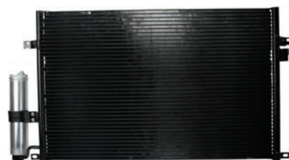
260730 Condenser Replacing: 96837834, 96484931 Servicing: Chevrolet, Daewoo Dryer w/ A: 406.00 B: 642.00 C: 20.00 mm
