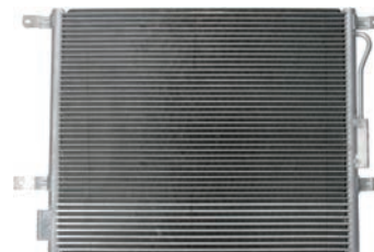
260409 Condenser Replacing: 55116931AA Servicing: Jeep Dryer w/o A: 465.00 B: 580.00 C: 28.00 mm
