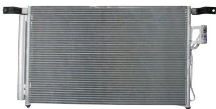
260400 Condenser Replacing: 976062B200, 97606-2B200, 97606-2B000, 260940 Servicing: Hyundai Dryer w/ A: 440.00 B: 715.00 C: 20.00 mm
