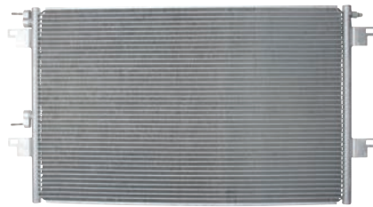
260462 Condenser Replacing: 8200332851 Servicing: Renault Dryer w/o A: 430.00 B: 690.00 C: 20.00 mm
