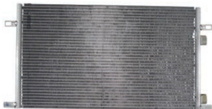
260459 Condenser Replacing: 7701045346, 7701038395 Servicing: Renault Dryer w/o A: 358.00 B: 640.00 C: 20.00 mm
