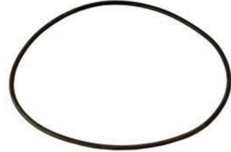
250785 O-ring ID 116.00, Thickness 2.50, Material Nioprene
