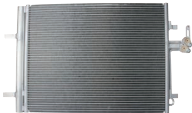
260916 Condenser Replacing: 31274157, 30794562 Servicing: Volvo Dryer w/ A: 472.00 B: 625.00 C: 20.00 mm
