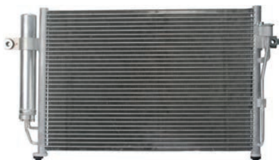
260914 Condenser Replacing: 97606-1C100, 97606-1C000 Servicing: Hyundai Dryer w/ A: 365.00 B: 542.00 C: 22.00 mm
